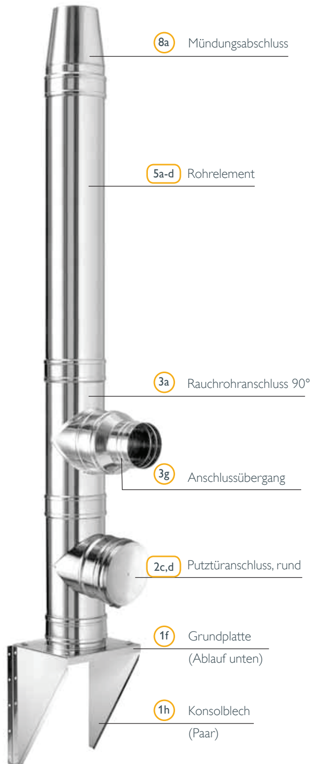
Wandmontage
