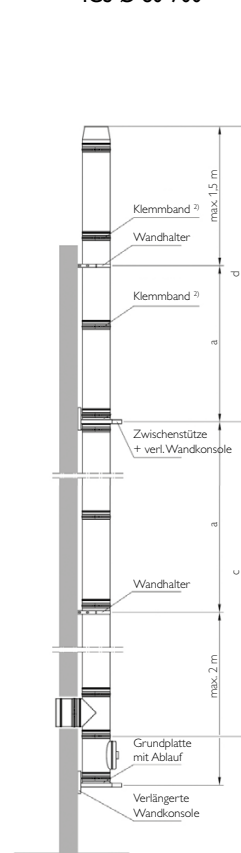
ICS Ø 80-700
