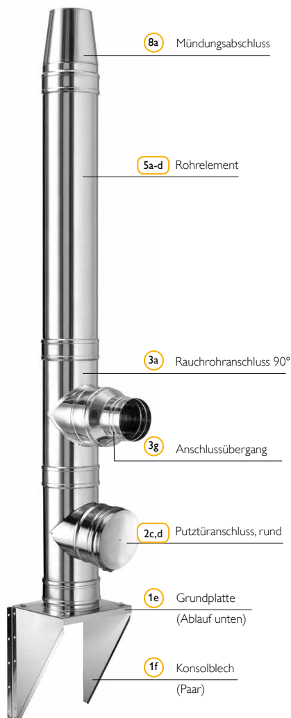
Wandmontage
