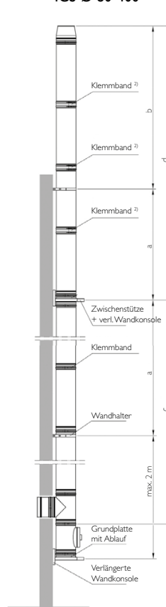
ICS Ø 80-400
