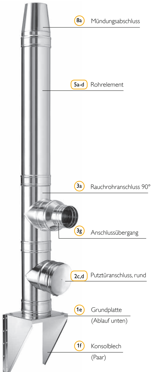
Wandmontage
